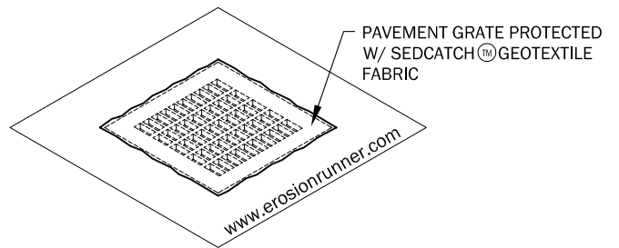
SedCatch™ Pavement Grate
