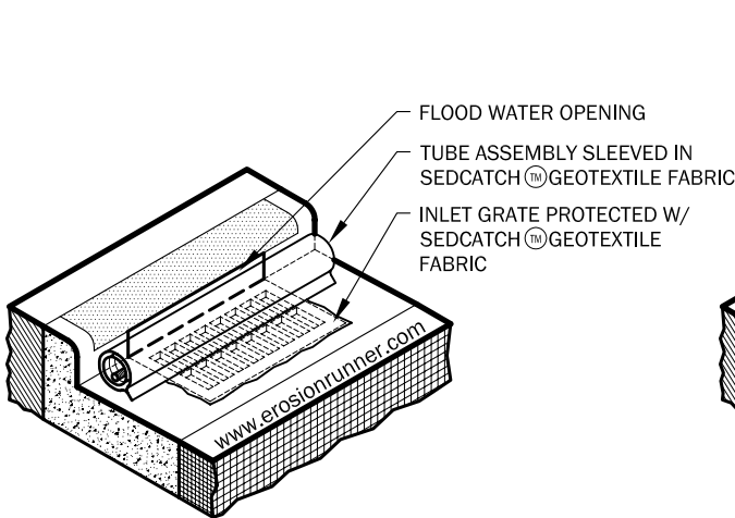
SedCatch™ Curb & Gutter
