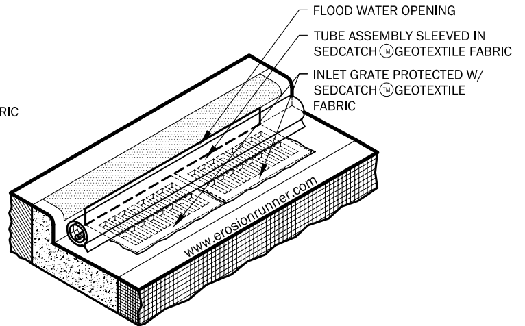
SedCatch™ Double Curb & Gutter
