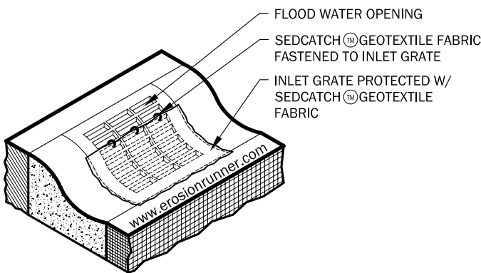
SedCatch™ Rolled Curb Grate
